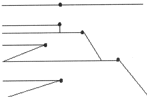
Figure 2: polar diagram of 6 points
