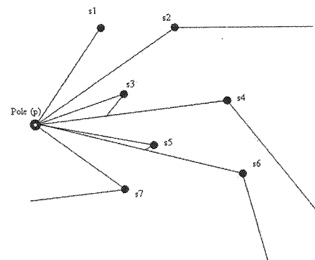
Figure 4: Near pole polar diagram of 7 points
