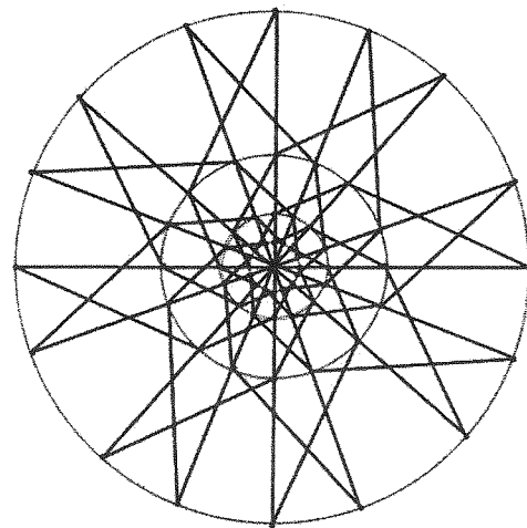
Figure 9: NPPD (in two directions) for the sites in Figure 8.
